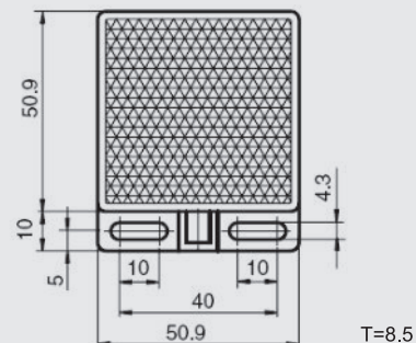
RB50x50 (optional)
