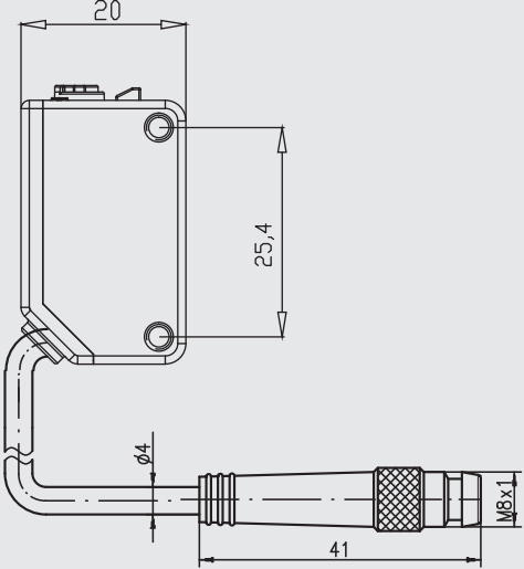
M8 connector
