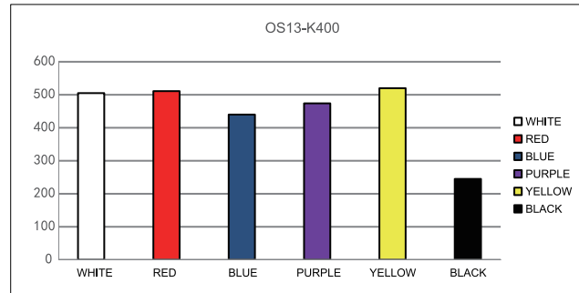
OS13-K400 diffused attenuation figure
