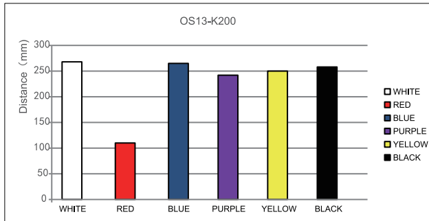
OS13-K200 diffused attenuation figure
