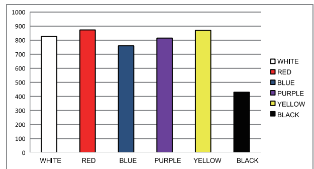
OP18-K600VP6 diffused attenuation figure
