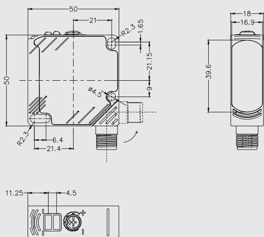
M12 connector
