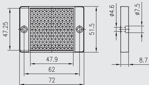
RB50x50-1 (standard)
