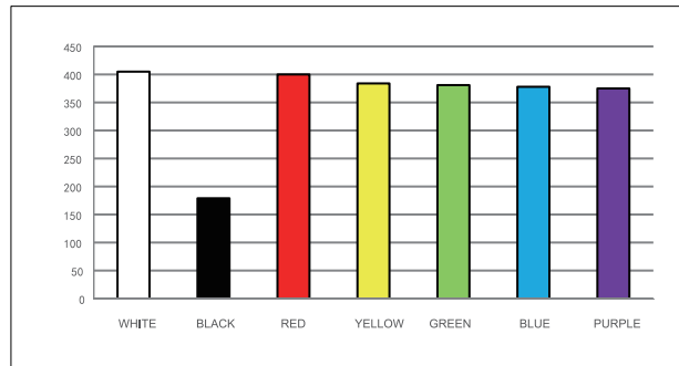
OS50-K7000VR5 diffused attenuation figure
