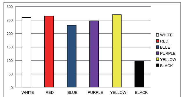
OM18-K200VP6 diffused attenuation figure
