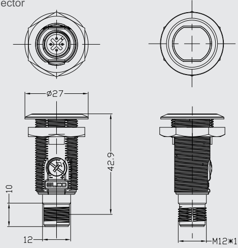
M12 connector
